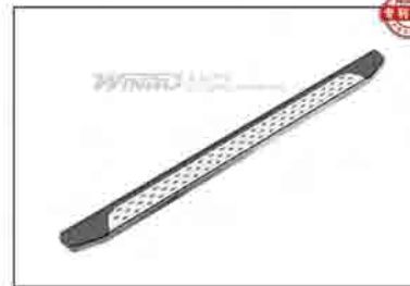
PW001689 76" AL. RUNNING BOARD FOR VEHICLE W/ FENDER TRIM M16 BRACKETS PW006532 (H240902A1) DOUBLE CAB:
